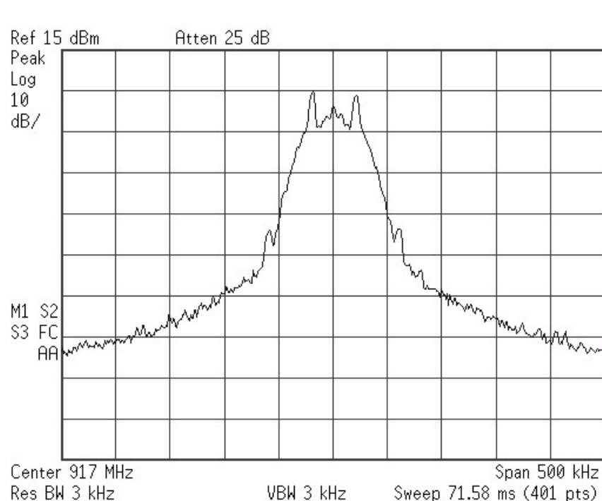
Figure 36. TX Modulated Spectrum (917 MHz, 40 kbps, 20 kHz Deviation, GFSK)
